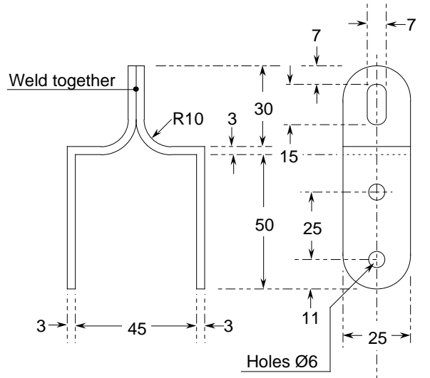
MAIN SHEET LOWER STRAP Scale 1/2
